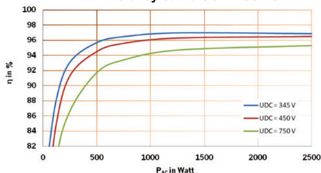
Efficiency curve SOLPLUS 25
